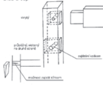
Dlab a čep
